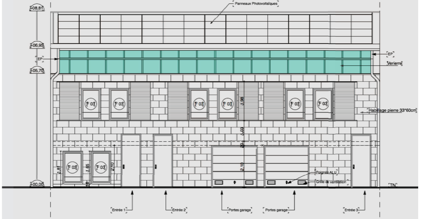
FACADE SUD
