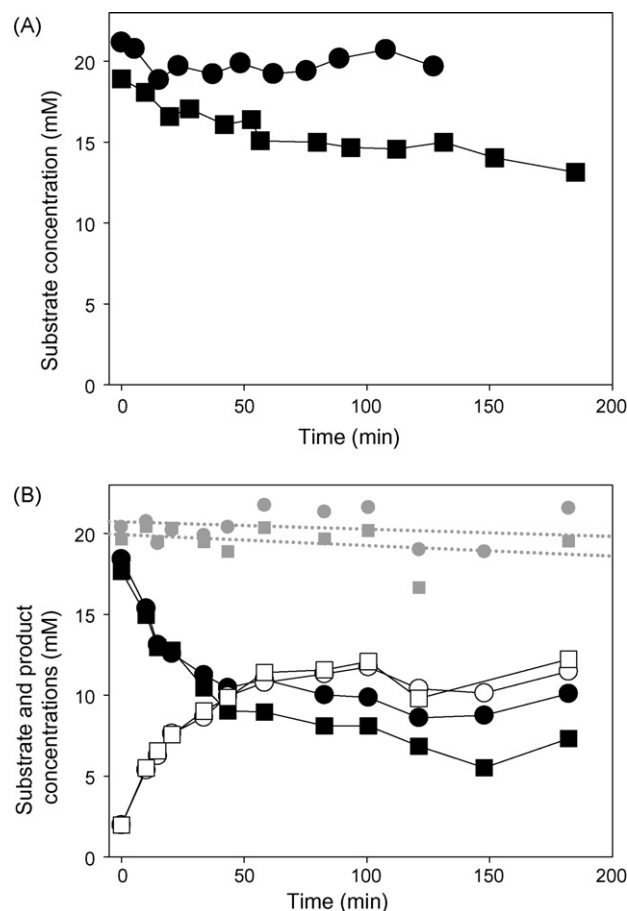
Fig. 1. Coupled oxidation–reduction of 1-butanol–hexanal by 1-butanol-grown Rhodococcus erythropolis NCIMB 13064 cells in aqueous batch conditions (40 °C, pH 7.0). (A) 1-Butanol (●) or hexanal (■) were added separately to the fresh cell suspension (OD 690 nm = 0.78). (B) 1-Butanol (●) and hexanal (■) were added together to the cell suspension (OD 690 nm = 0.78) allowing the production of butanal (○) and 1-hexanol (□). Total concentrations of C4- (●) and C6- (■) compounds are shown together with linear regressions (dotted lines). C4- and C6-acids were not produced at detectable levels. Data are means of at least two GC determinations.
