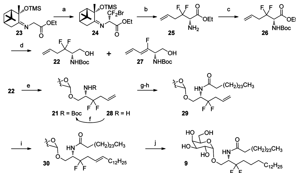
Scheme 4. Synthesis of 3,4-Dideoxy-3,3-difluoro Analogue 9 a
