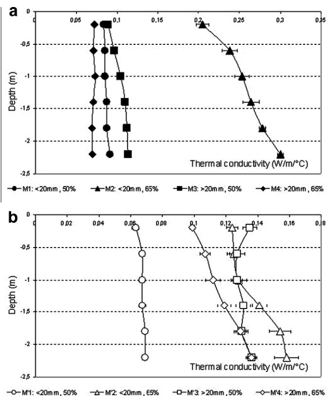
Fig. 5. Thermal conductivity as a function of depth at different moisture contents and particle sizes (a: sludge–recycled palettes mixtures; b: sludge–fresh palettes mixtures).
