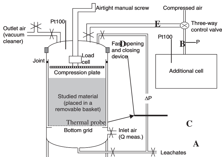
Fig. 1. Schematic representation of the “CPP” device.
