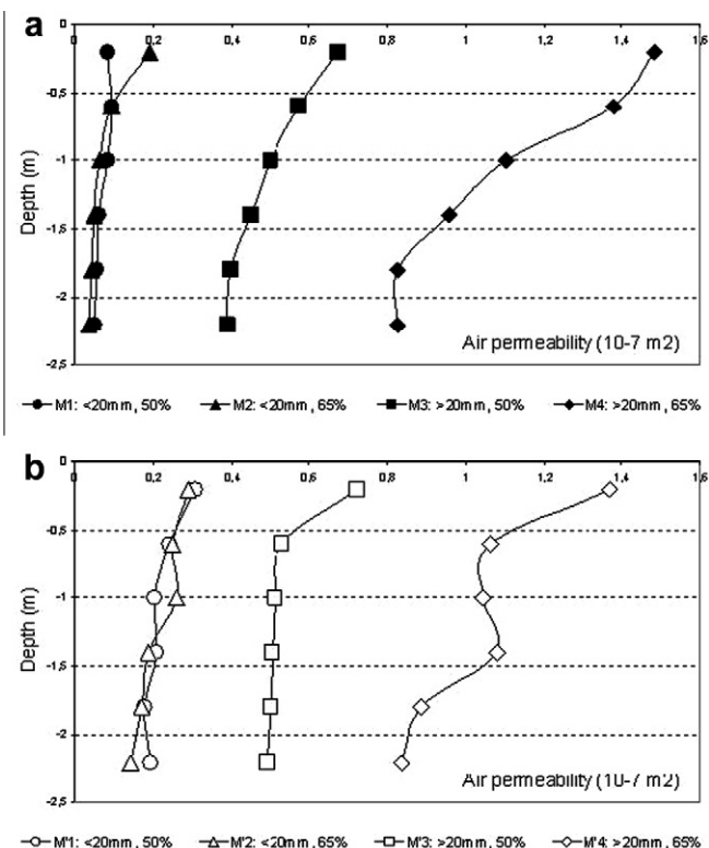
Fig. 4. Air permeability as a function of depth at different moisture contents and particle sizes (a: sludge–recycled palettes mixtures; b: sludge–fresh palettes mixtures).
