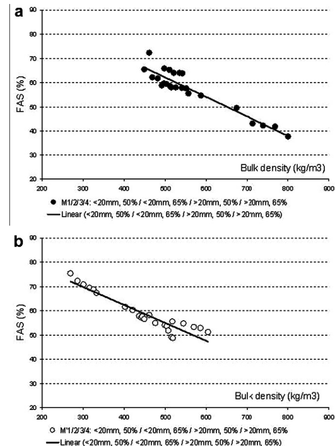
Fig. 6. FAS as a function of bulk density at different moisture contents and particle sizes (a: sludge-recycled pallettes mixtures; b: sludge-fresh pallettes mixtures).
