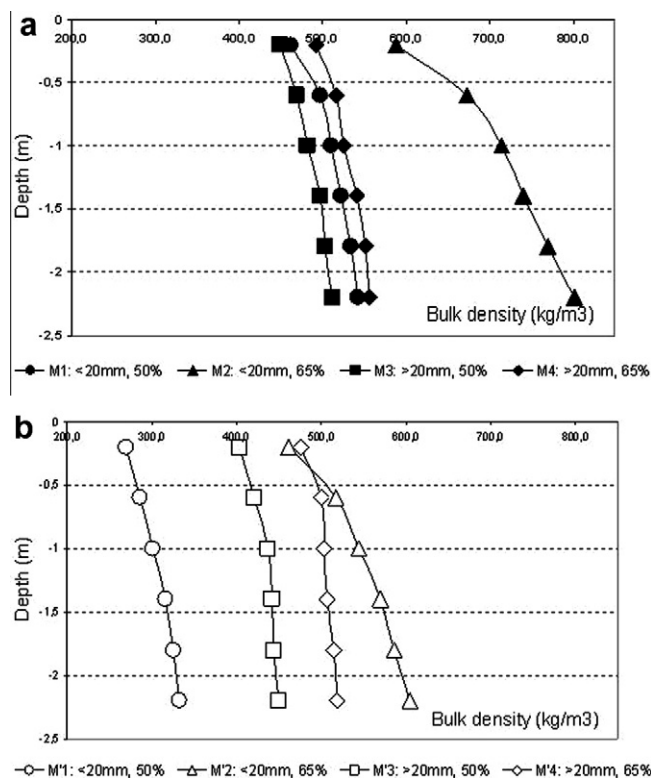
Fig. 2. Bulk density as a function of depth at different moisture contents and particle sizes (a: sludge-recycled palettes mixtures; b: sludge-fresh palettes mixtures).
