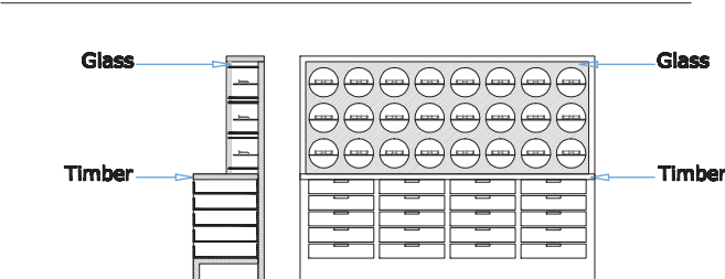
Back to Back Glasses Display with drawers - 1/50
