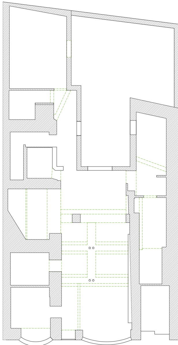
Ceiling Plan
