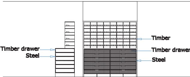
Back to Back Glasses Display with drawers - 1/50
